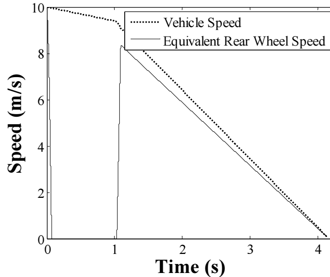
Fig. 20. Vehicle and equivalent rear wheels speed on complex road condition, RBS-noABS
