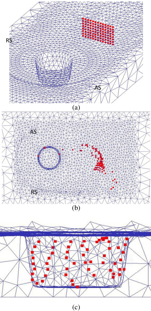
Fig12. (a) Initial position of points in front of tool which were picked for specification of overall material flow pattern, (b) and (c) final position of points.
