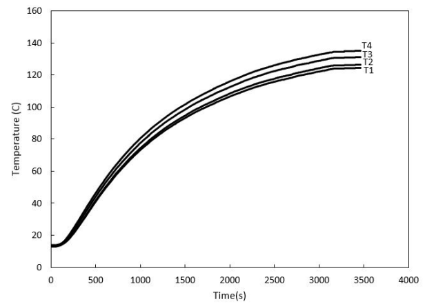
Figure 6. Temperature distribution for fix contact
