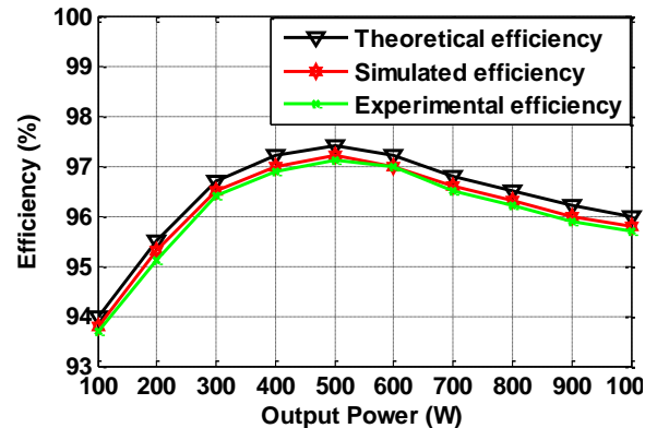
Figure 9: Comparison theoretical efficiency and the efficiency curve obtained from the simulation and experimental results.
