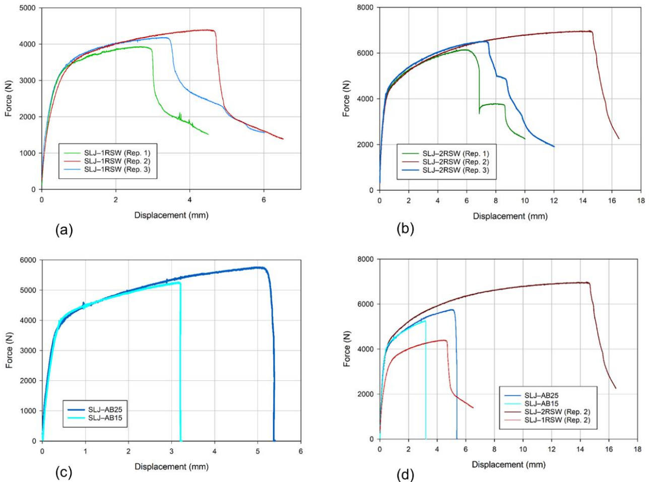
Figure 2: Force–displacement responses of single-lap joints (SLJs).
