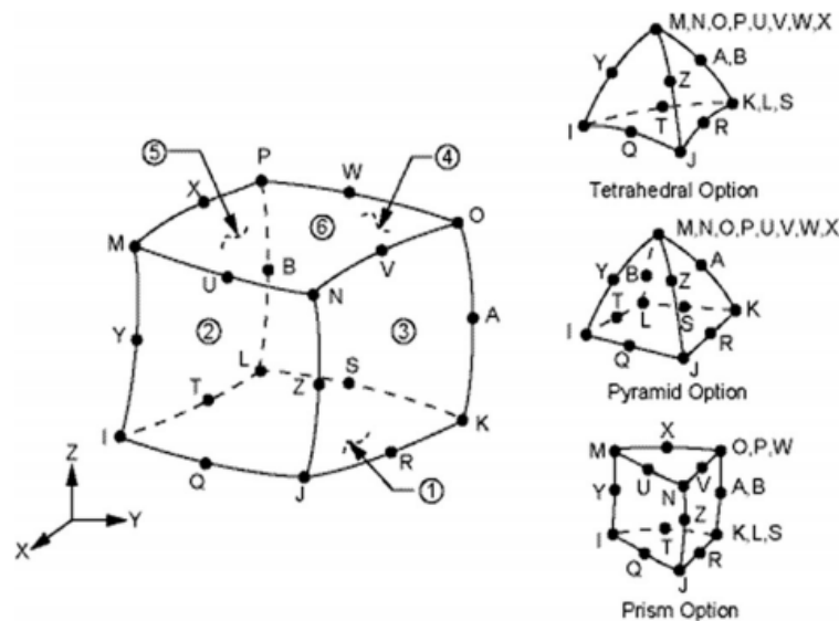
Fig. 3. Three dimensional thermal solid element SOLID226 [36].
