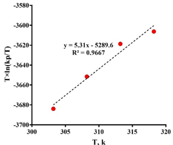
Fig. 11. Eyring equation for CuFeS 2 dissolution using experimental data.
