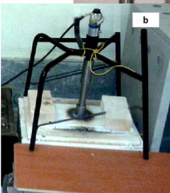
Fig. 4. a) Ultrasonic probe and (b) mechanical stirrer and ultrasonic device.
