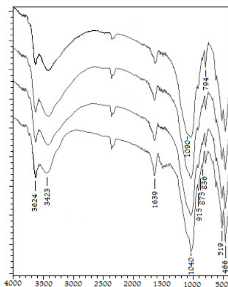
Fig. 3. FT-IR spectra of the natural and some acid activated samples.
