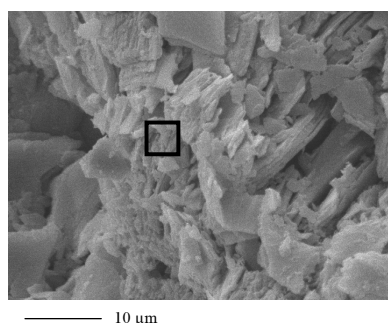
Fig. 21. Probable presence of very fine needle-like ettringite crystals, EDAX analysis (wt %); CaO: 62.78, SO 3 : 8.83, Al 2 O 3 : 3.05, SiO 2 : 18.16
