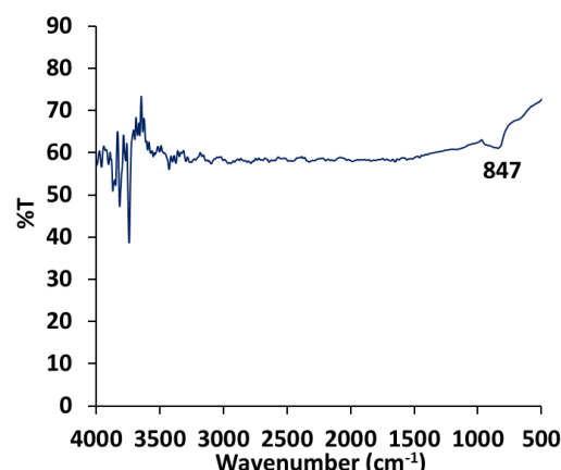
Fig. 4. Infrared Fourier transform curve of silicon carbide nanoparticles
