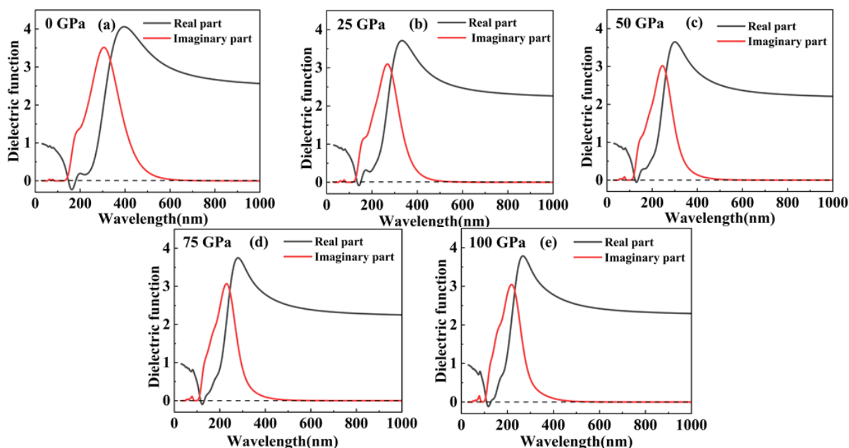
Fig. 11. The calculated dielectric function of \text{Ce}_{0.75}\text{Mo}_{0.25}\text{O}_2 at varying pressures
