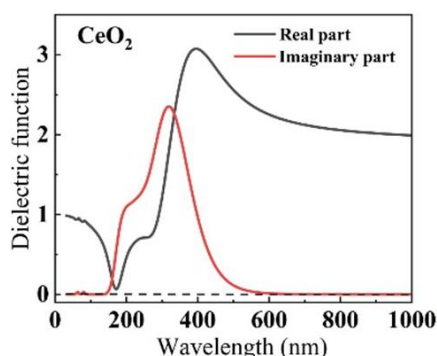
Fig. 10. The calculated dielectric function of \text{CeO}_2 at 0 GPa
