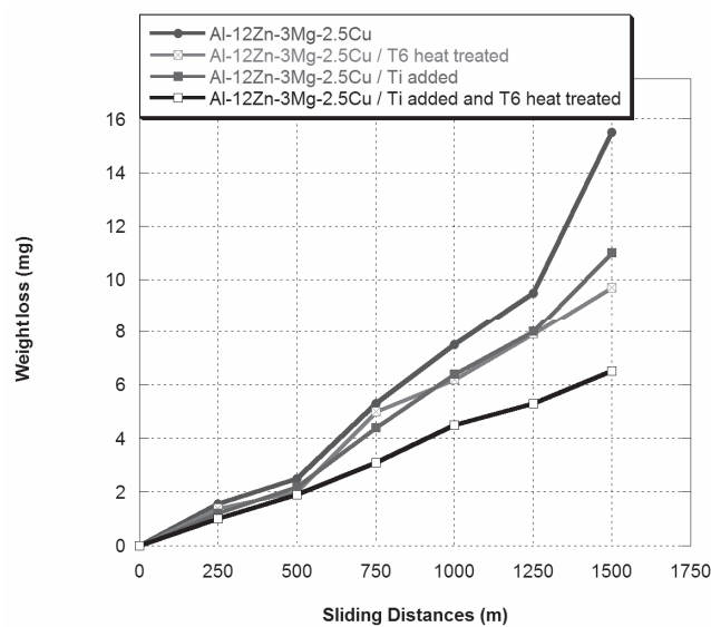
Fig. 7. Weight loss as a function of sliding distance for unrefined and 0.1% Ti-refined specimens with and without heat treatment.
