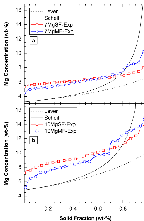
Fig. 9. Experimental concentration profiles of (a) 7Mg and (b) 10Mg alloy.
