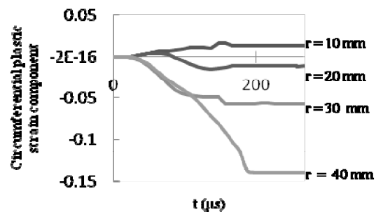
Fig. 16. Circumferential plastic strain versus time in different radii.
