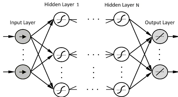
Figure 1: Architecture of the MLP model
